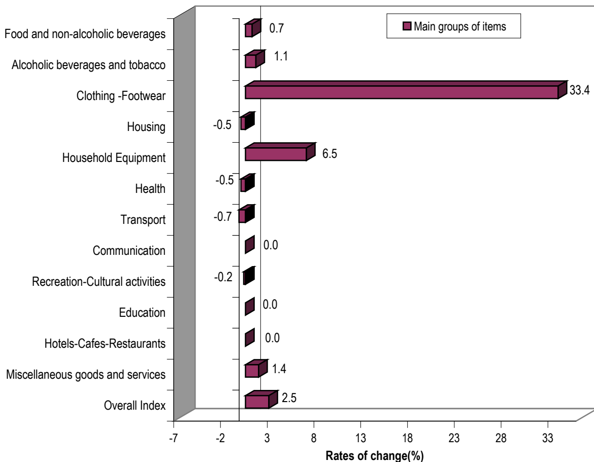
Annual rates of change (%) of the CPI between March 2013 and March 2012
