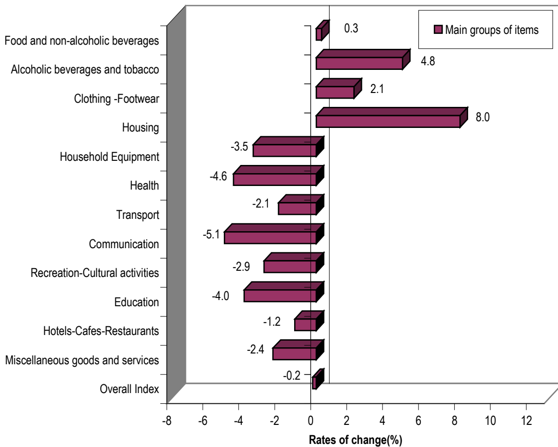
Annual rates of change (%) of the CPI between March 2013 and March 2012
