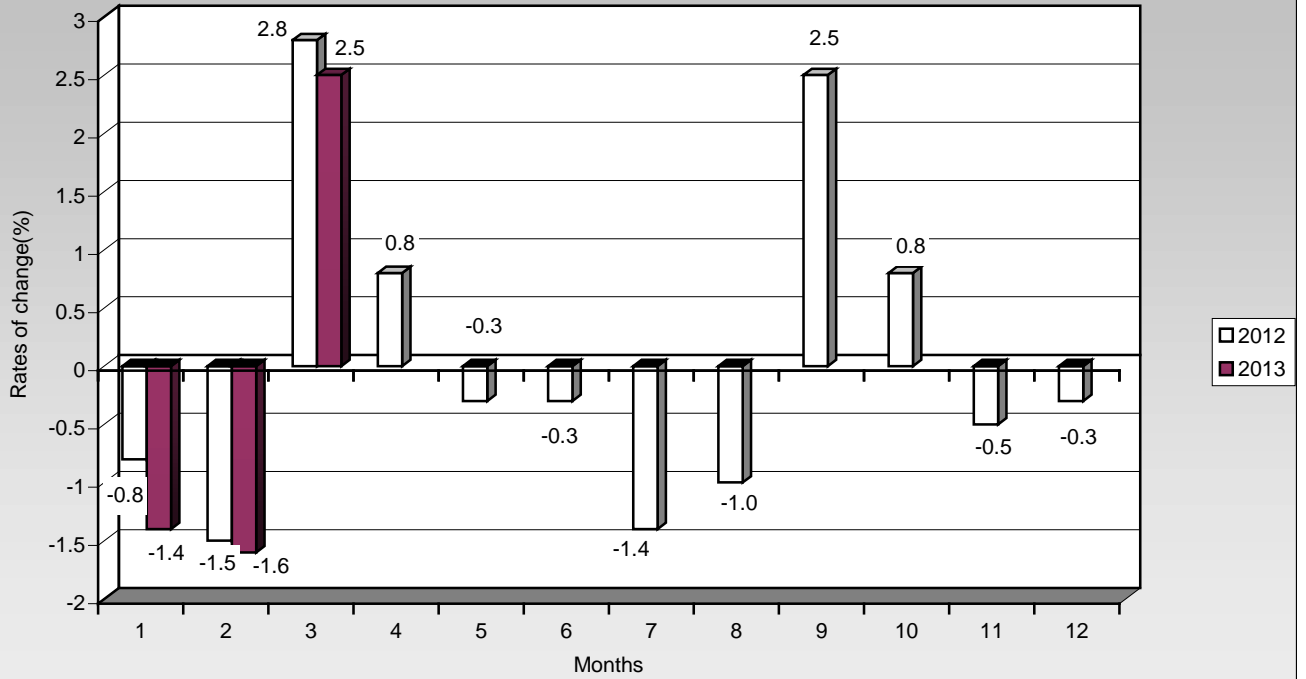
Monthly rates of change (%) of the overall Consumer Price Index during the years 2012 and 2013
