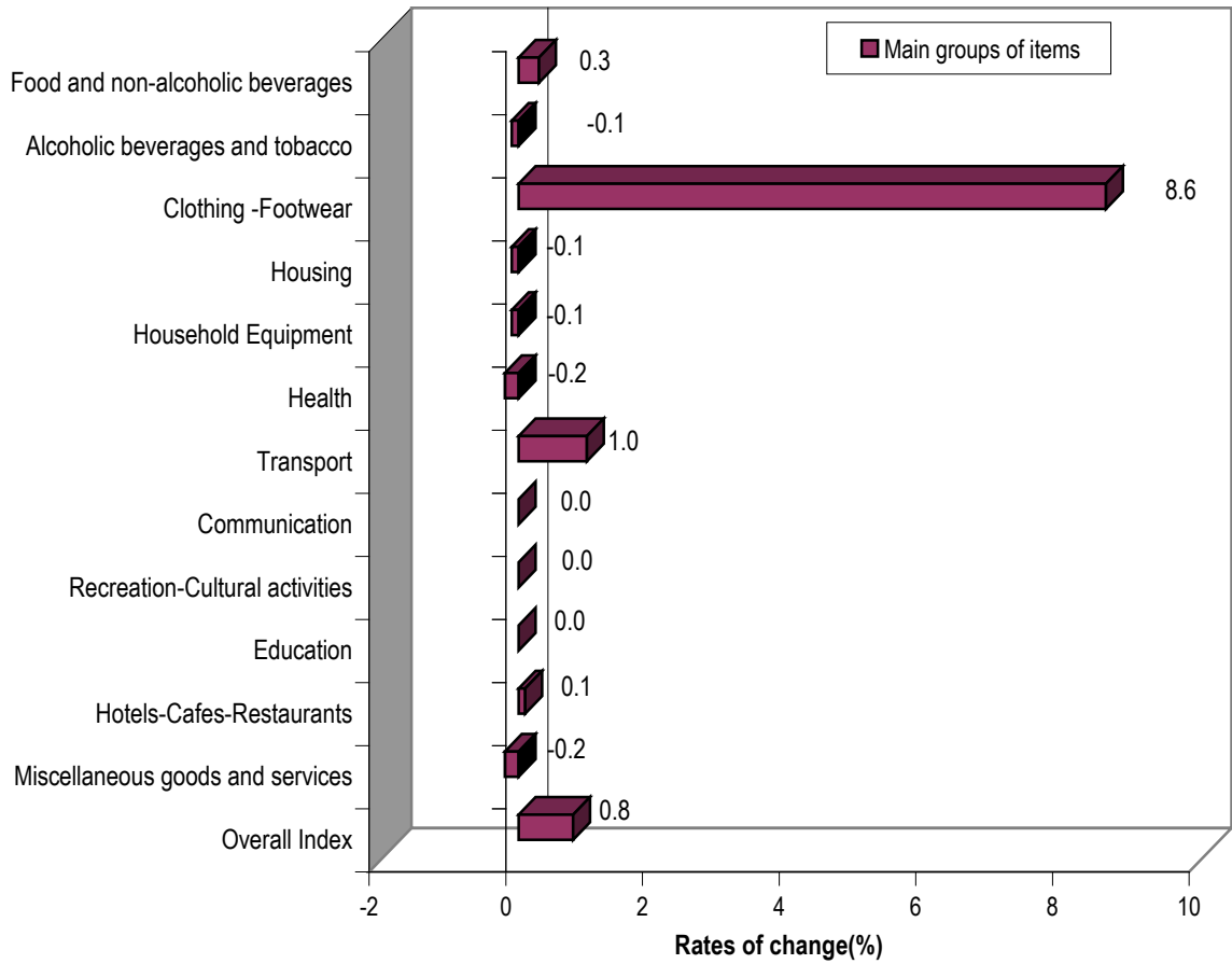
Annual rates of change (%) of the CPI between April 2012 and April 2011
