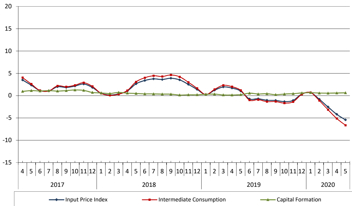
Graph 5. Annual rates of changes (%) of the Input Price Index in Agriculture – Livestock and of the sub-indices of Intermediate Consumption and Capital Formation (2015=100.0)
