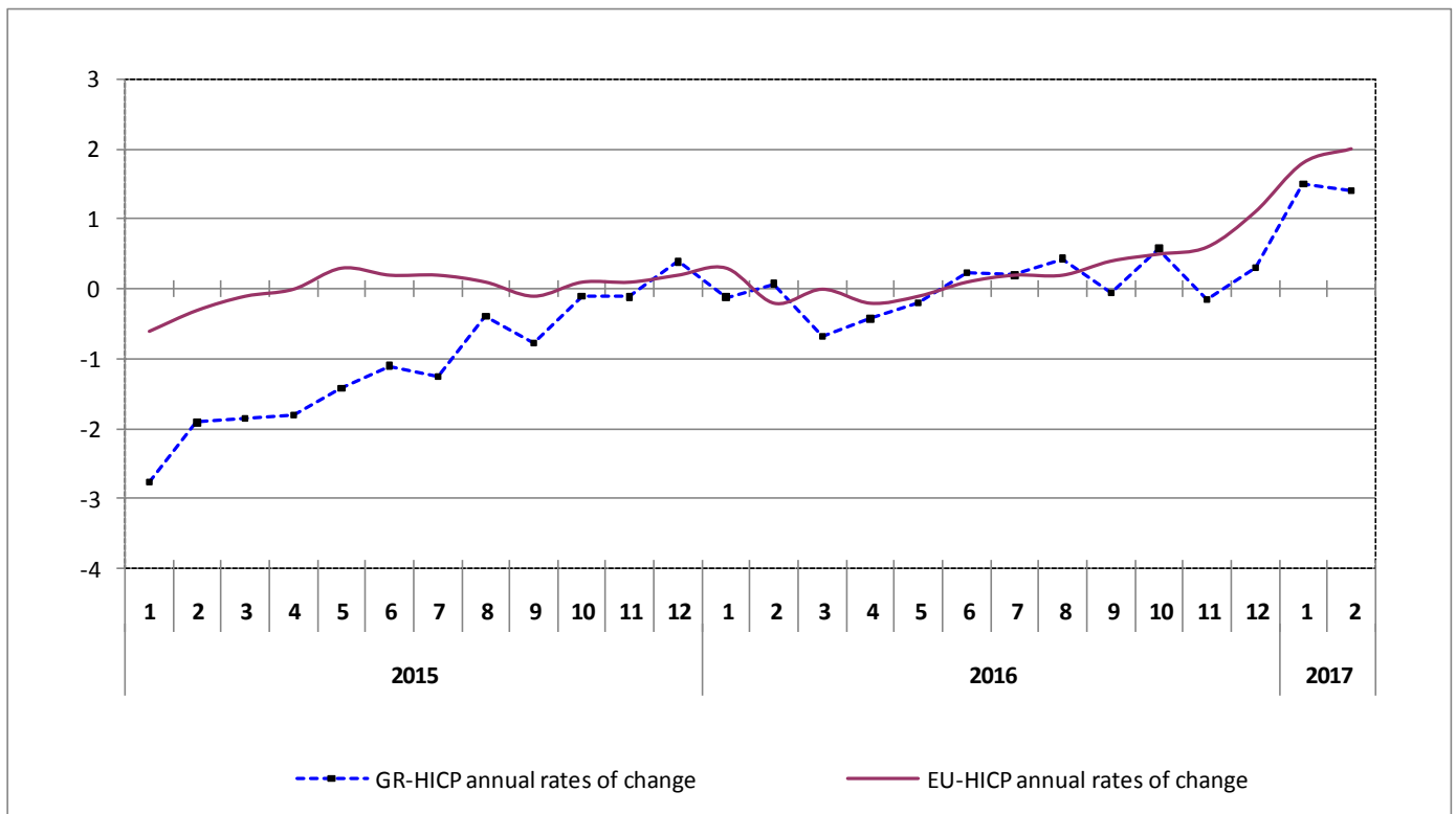
Annual rates of change (%) of GR-HICP and EU-HICP
