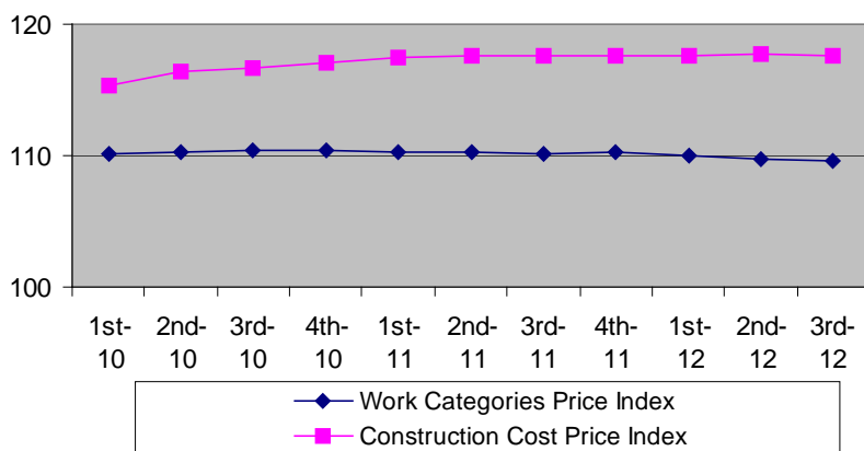
Evolution of Work Categories and Construction Cost Price Indices in construction of new residential buildings 2005=100.0
