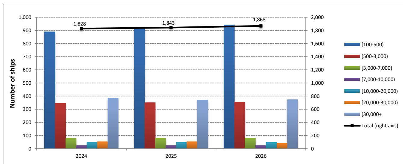
Graph 3: Distribution of Greek Merchant ships of 100 GRT and over, by tonnage groups, July 2024 – 2026
