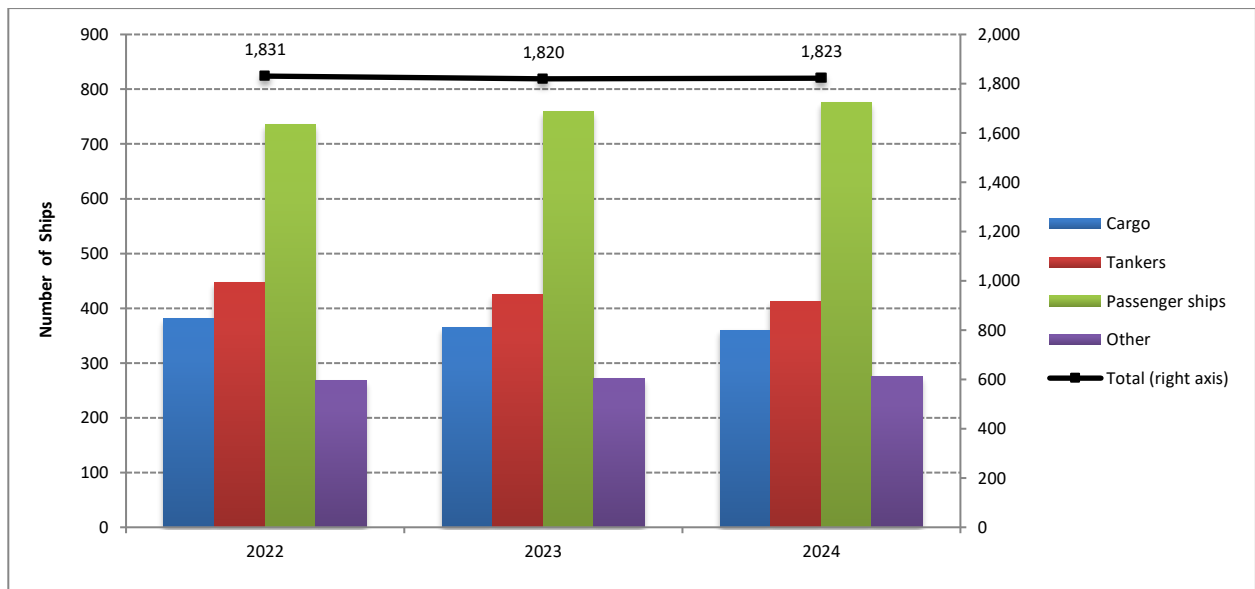
Graph 2a: Number of Greek Merchant ships of 100 GRT and over, by types of ships, May 2022 – 2024
