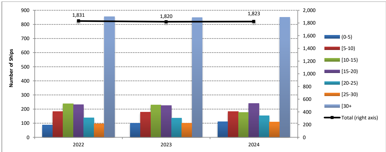
Graph 4a: Distribution of Greek Merchant ships 100 GRT and over, by age groups, May 2022 – 2024
