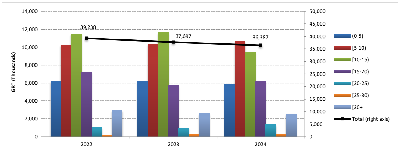
Graph 4b: Tonnage of Greek Merchant ships of 100 GRT and over, by age groups, May 2022–2024
