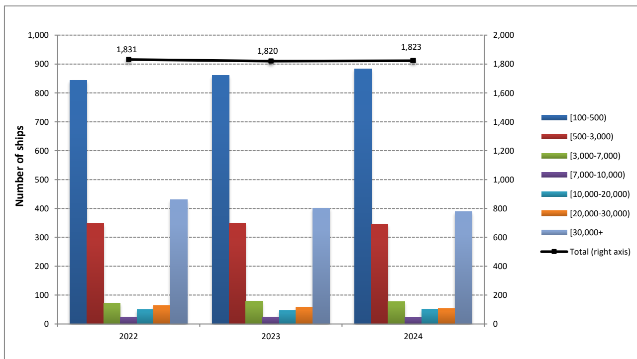
Graph 3: Distribution of Greek Merchant ships of 100 GRT and over, by tonnage groups, May 2022 – 2024
