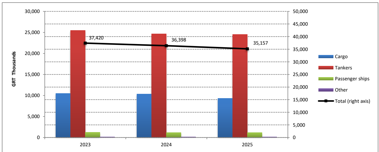
Graph 2b: Tonnage of Greek Merchant Ships of 100 GRT and over, by types of ships, June 2023 – 2025
