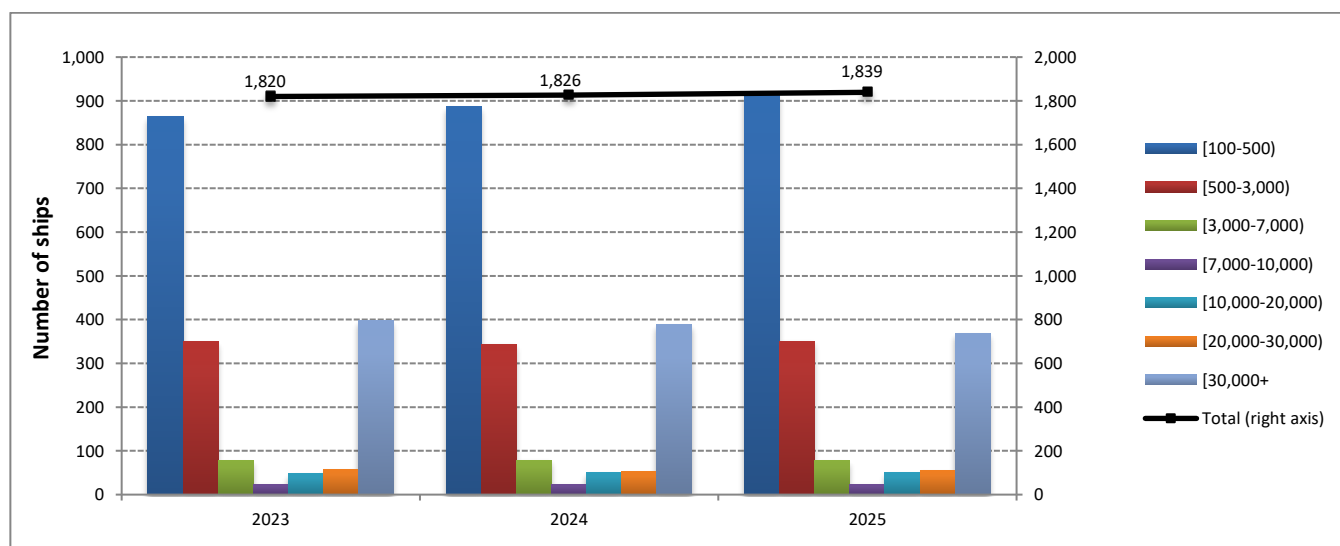
Graph 3: Distribution of Greek Merchant ships of 100 GRT and over, by tonnage groups, June 2023 – 2025
