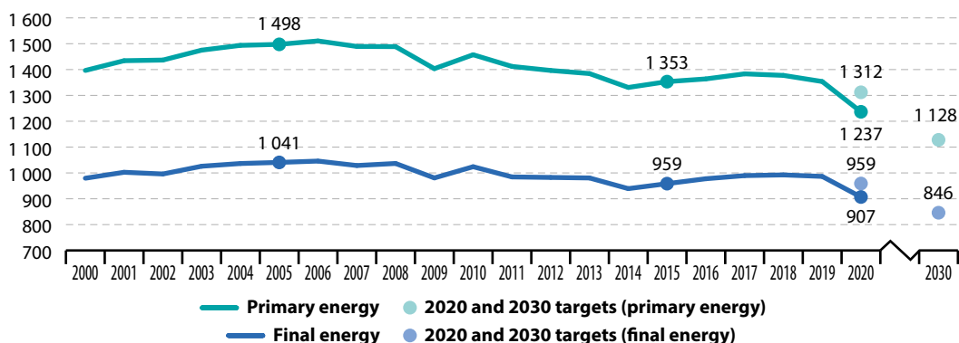
Figure 7.1: Primary and final energy consumption, EU, 2000–2020 (million tonnes of oil equivalent (Mtoe))
