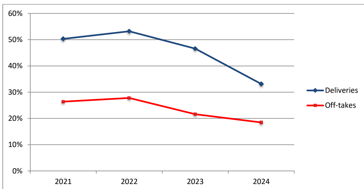
Graph 3. Percentage share of natural gas deliveries and off-takes at entry-exit points of the NNGS in relation to their technical capacity (%), 2021-2024
