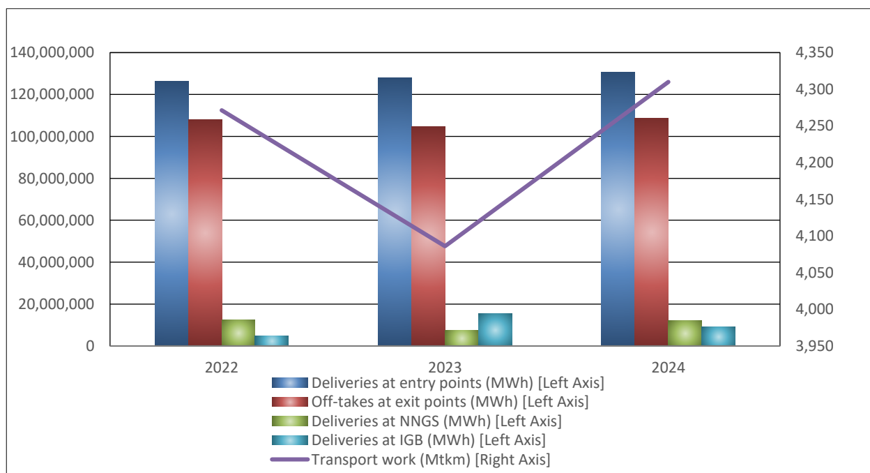
Graph 4. Natural gas transport via TAP, 2022 - 2024
