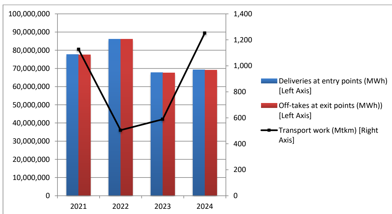
Graph 2. Transmission of natural gas through the NNGS, 2021-2024
